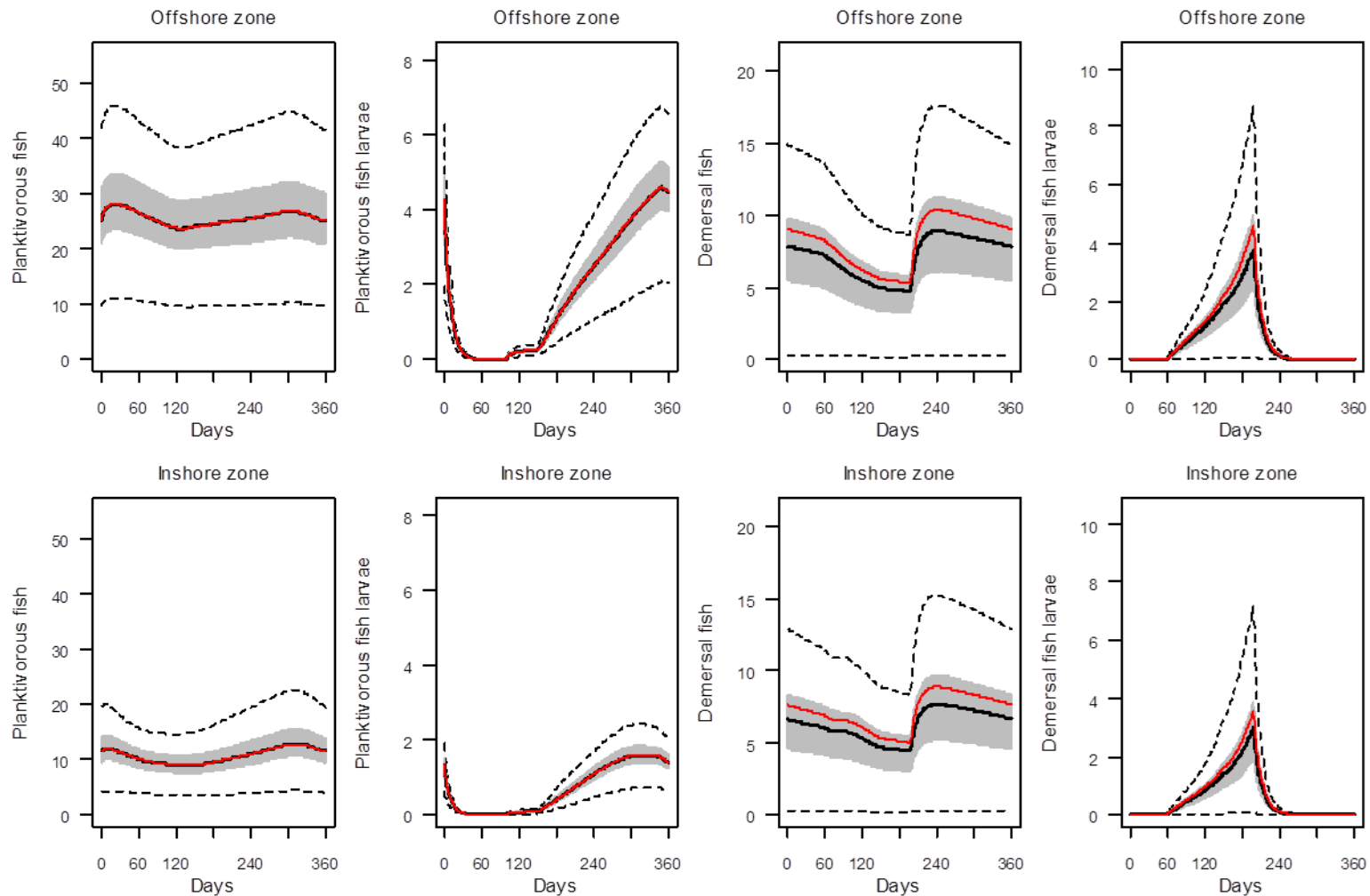
FIGURE 19 Stationary annual cycles of planktivorous and demersal fish guilds and their larval stages for the 1970-1999 fitted model. Dashed lines span the 99% likelihood interval of model outputs given the observed indices of the state of the North Sea during this period. Grey shading spans the 50% likelihood interval. Solid black line is the median of the likelihood distribution and the red line is the maximum likelihood model. Columns of panels are different variables output from the model, rows are different spatial compartments. Units for all variables: \text{mMN m}^{-2} .
