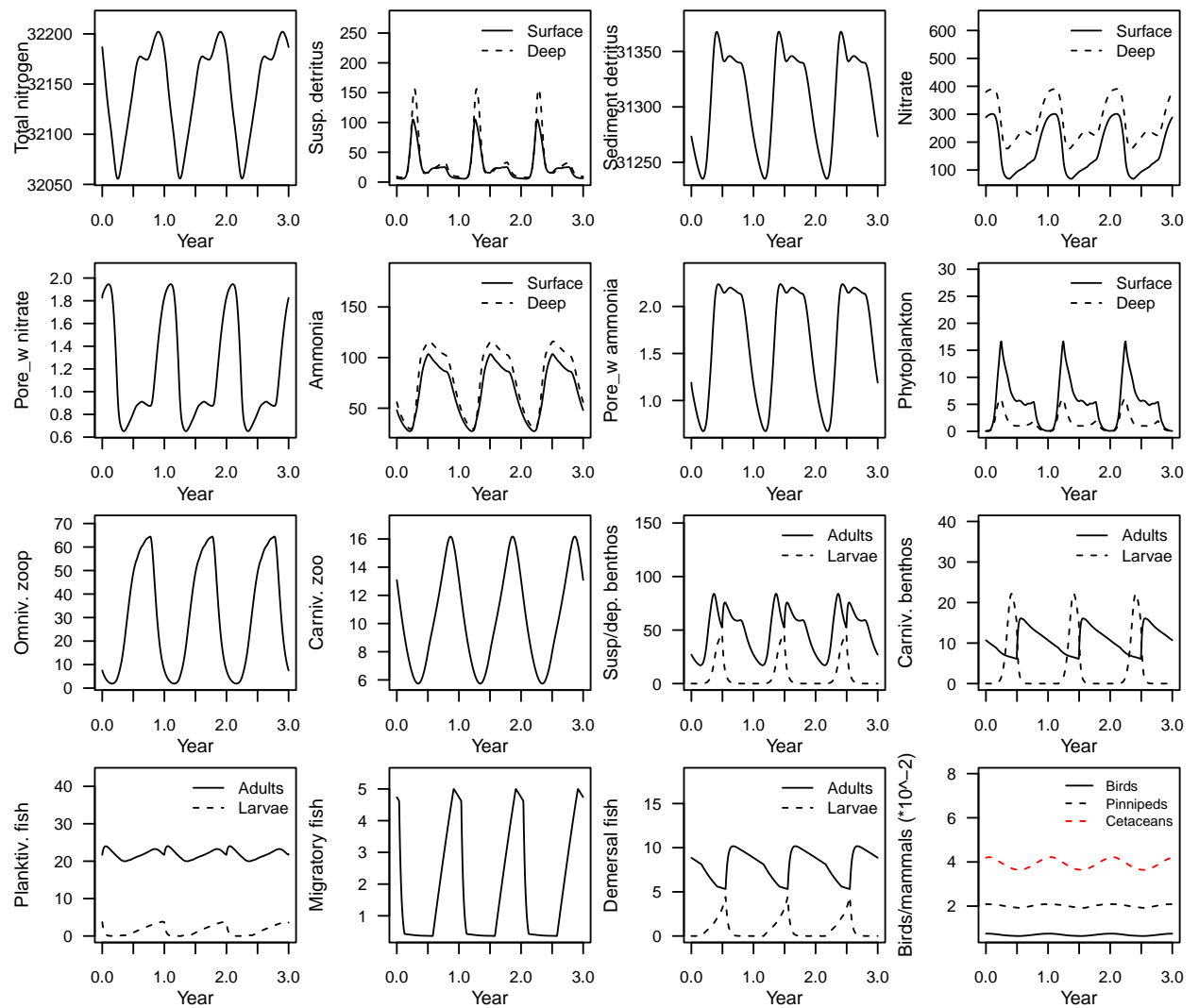
Figure 4. Time-series plot of ecology model output, units mMN in the model domain as a whole (1 m -2 sea
