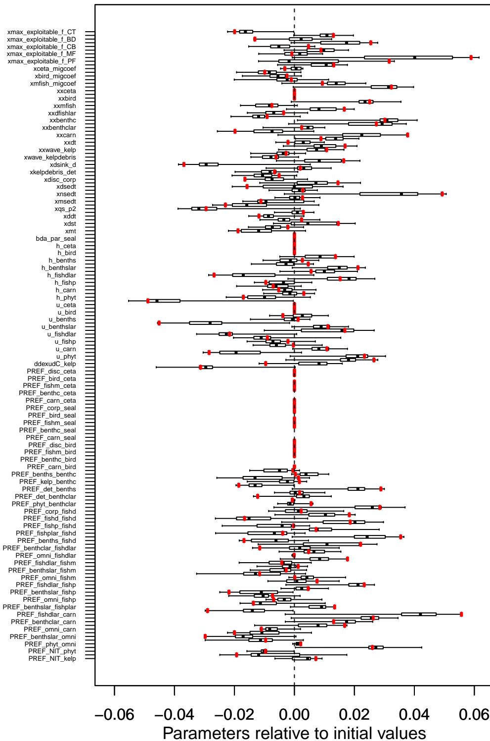
Figure 11. Diagnostic plot of the procedure from optimizing ecology model parameters for the North Sea 1970-1999 model.
