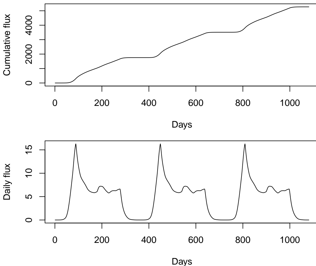
Figure 9. Upper panel: time series of the cumulative phytoplankton gross production as output from the model. Lower panel: same data converted into daily gross production rates.
