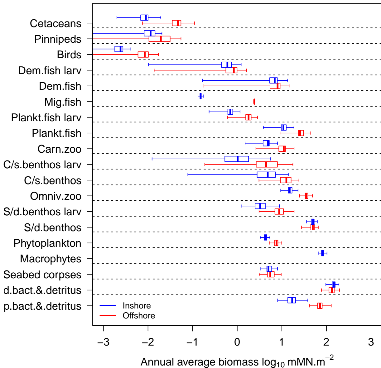
Figure 47. Annual average biomass densities with credible intervals for the final year of a single run of the 1970-1999 North Sea model.
