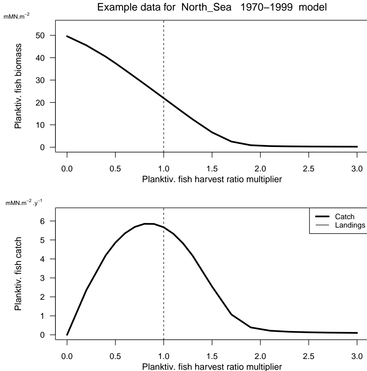
Figure 28. Yield data plot for planktivorous fish in the 1970-1999 North Sea model with baseline demersal harvest ratios. Upper panel, annual average biomass of planktivorous fish (mMN.m -2 in the whole model domain) as a function of harvest ratio. Lower panel: catch divided into landings and discards of planktivorous fish (mMN.m -2 .y -1 ) as a function of harvest ratio.
